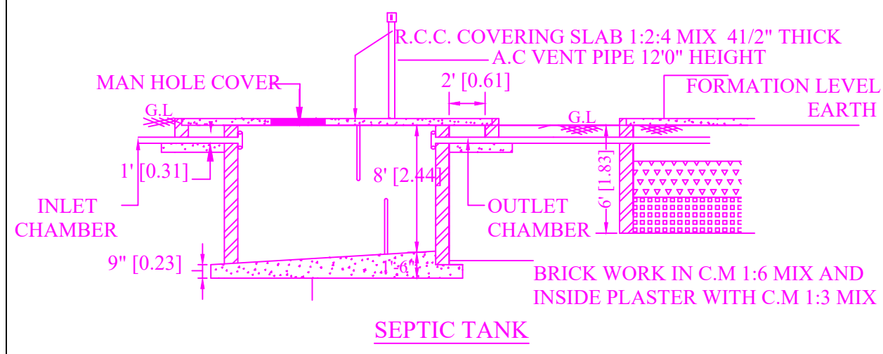
SEPTIC TANK
