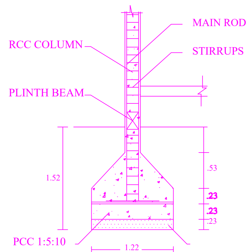
COLUMN DETAILS
