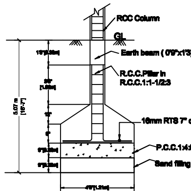
FOUNDATION DETAILS
