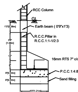
FOUNDATION DETAILS
