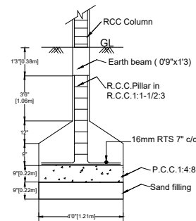
FOUNDATION DETAILS
