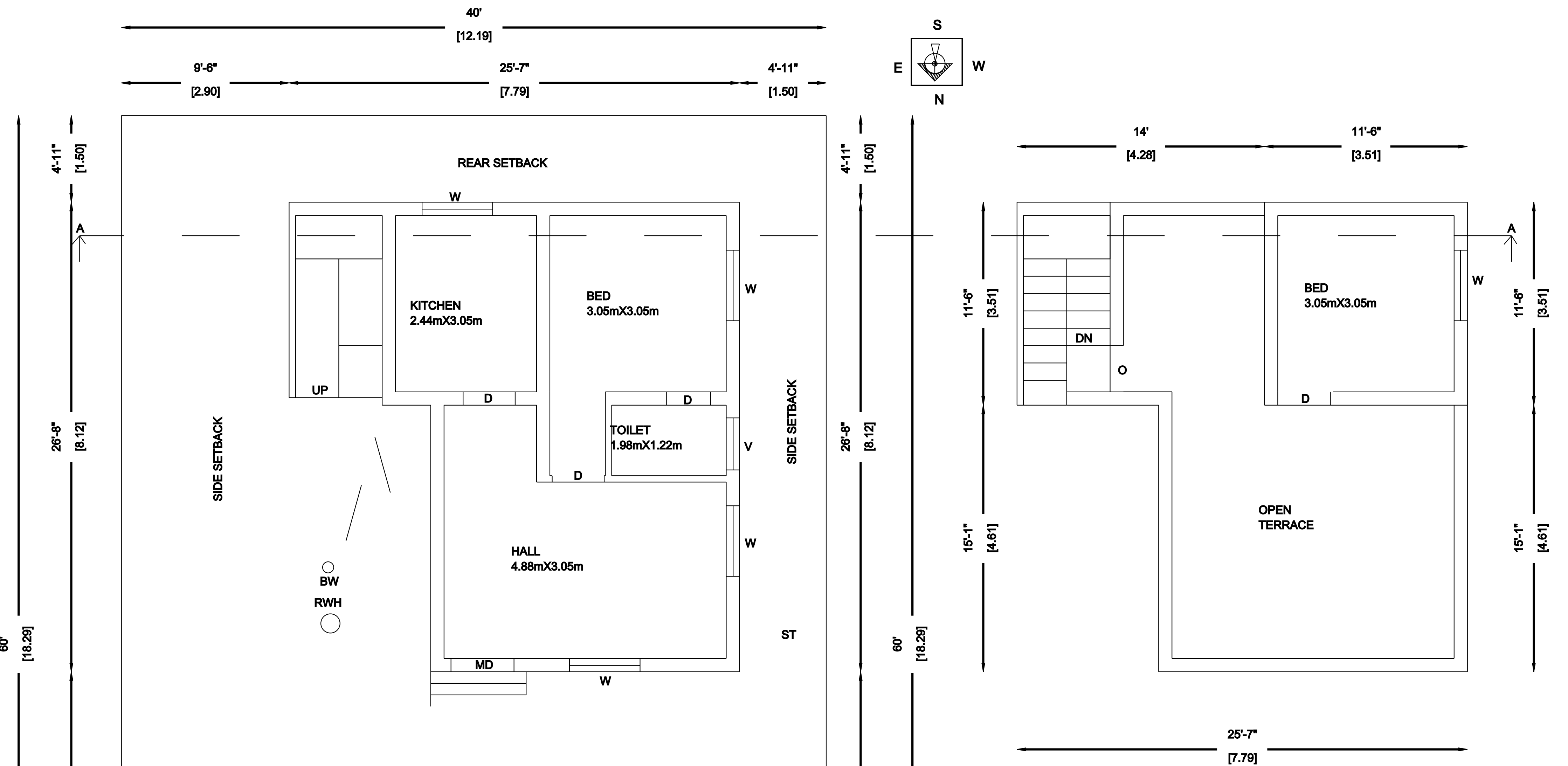
PRO. FIRST FLOOR PLAN
