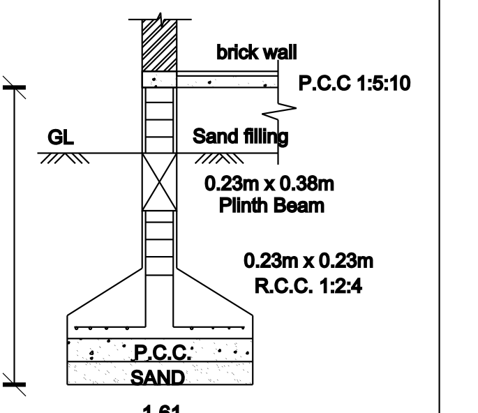
FOUNDATION DETAILS
