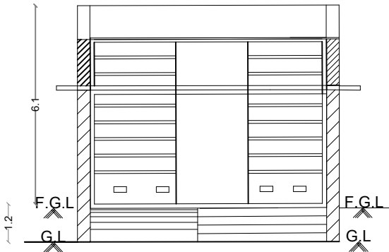
FRONT ELEVATION
