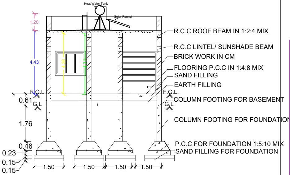
SECTION ON-AA
