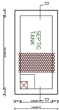
PLAN OF SEPTIC TANK SCALE 1"=2'0"
