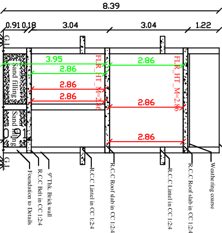
SECTION ON "RK"
