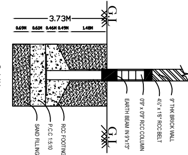
FOUNDATION DETAIL
