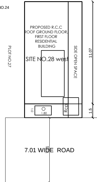
SITE PLAN
