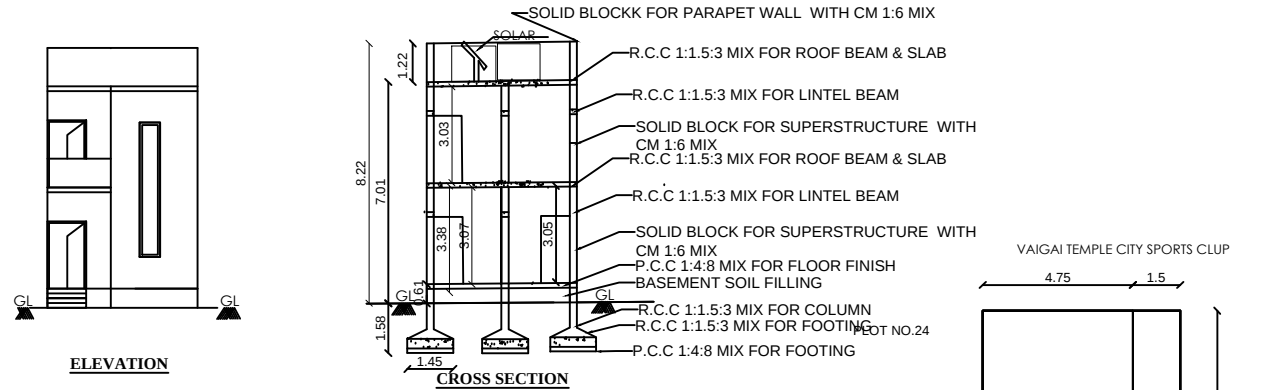
CROSS SECTION
