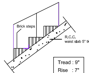
STAIRCASE DETAILS-NTS
