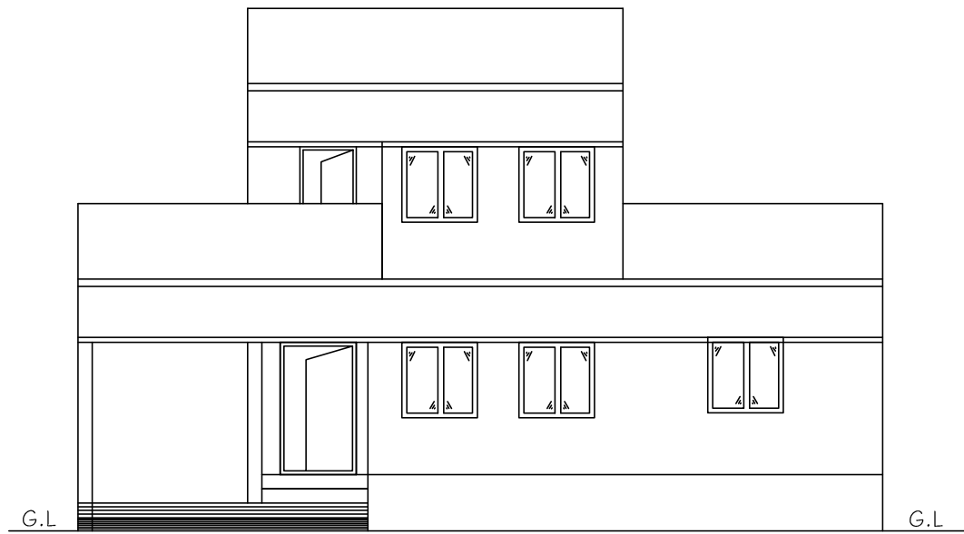
FRONT ELEATION
