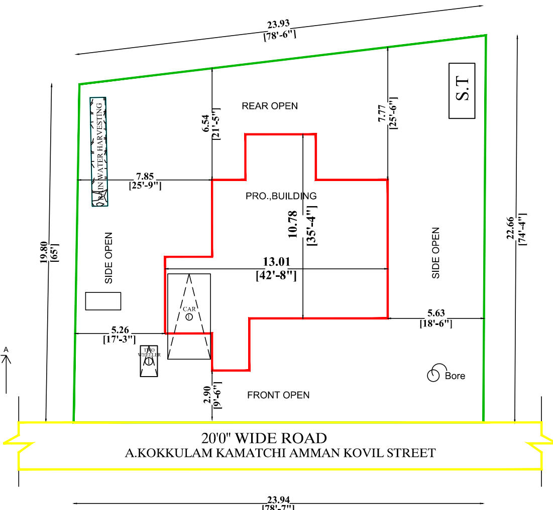
SITE PLAN
