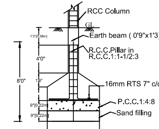
FOUNDATION DETAILS
