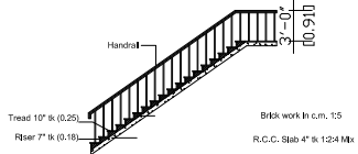
Staircase Details
