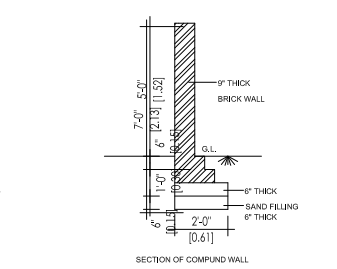
SECTION OF COMPOUND WALL
