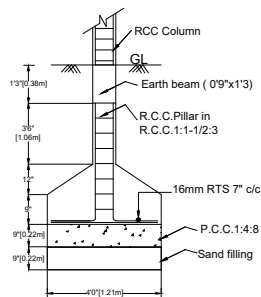
FOUNDATION DETAILS
