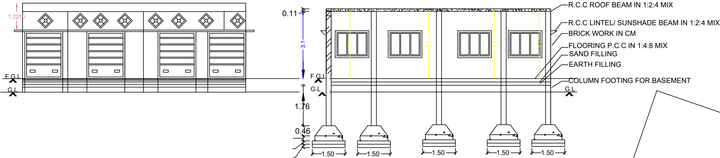
FRONT ELEVATION
