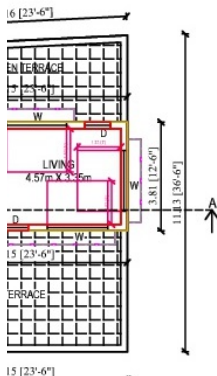
FLOOR PLAN
