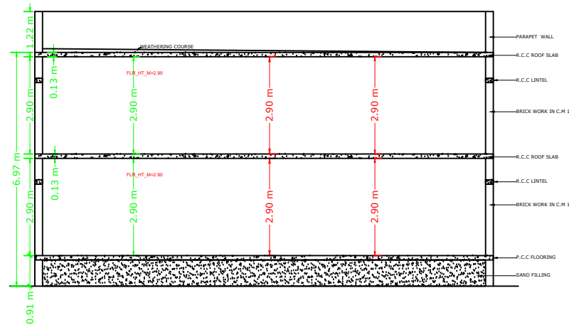
SECTION
