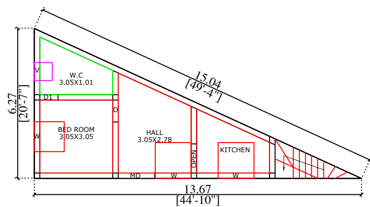
----- OR PLAN
