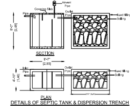
DETAILS OF SEPTIC TANK & DISPERSION TRENCH
