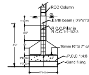
FOUNDATION DETAILS
