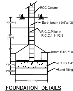
FOUNDATION DETAILS
