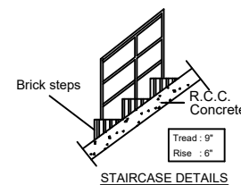
STAIRCASE DETAILS
