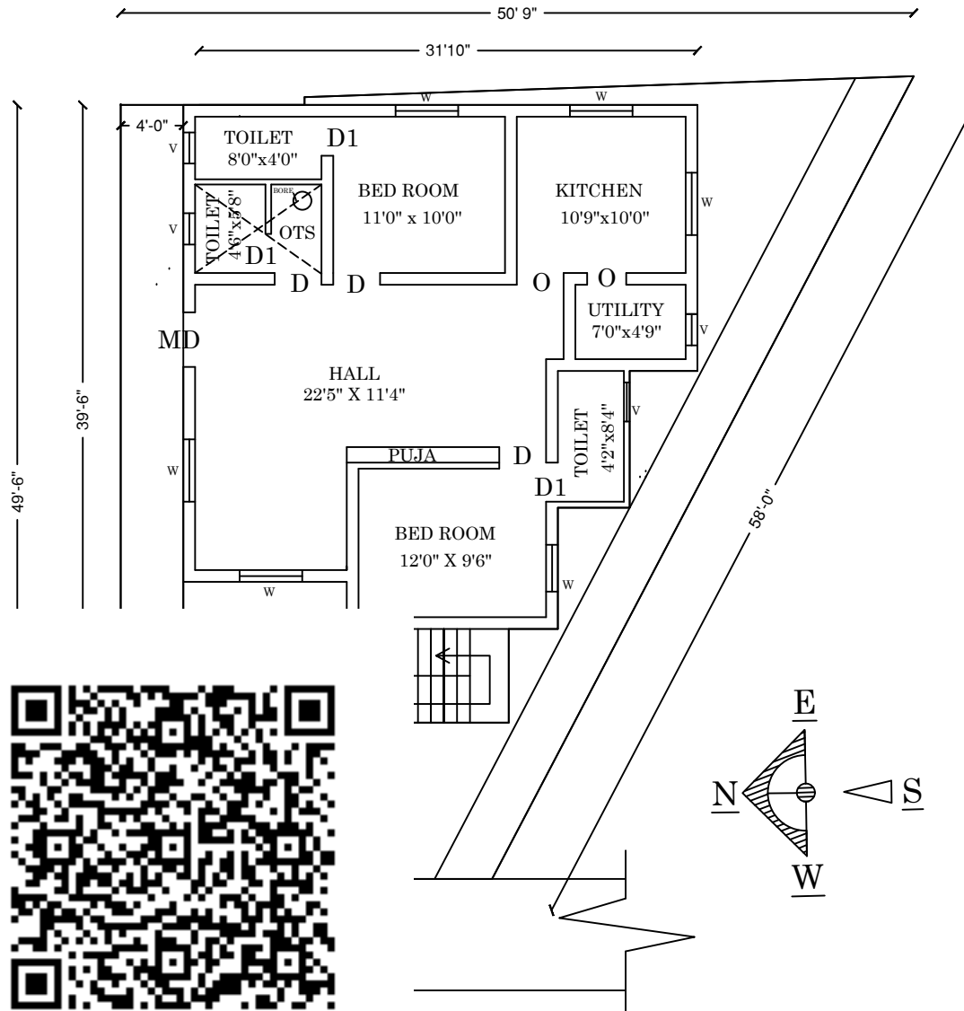
FIRST FLOOR PLAN FIRST FLOOR PLAN AREA= 1120 sq feet
