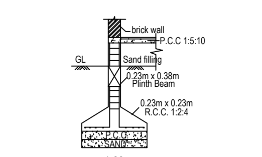
FOUNDATION DETAILS
