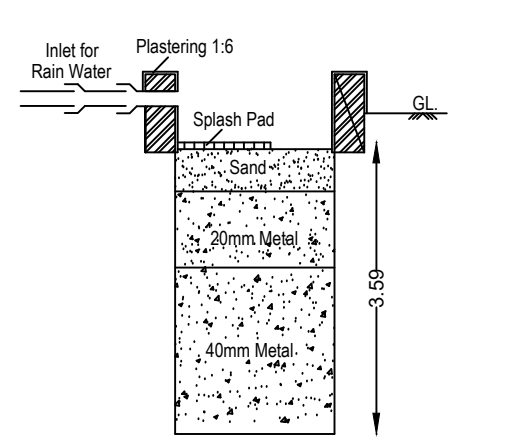
RAIN WATER PERCOLATION PIT
