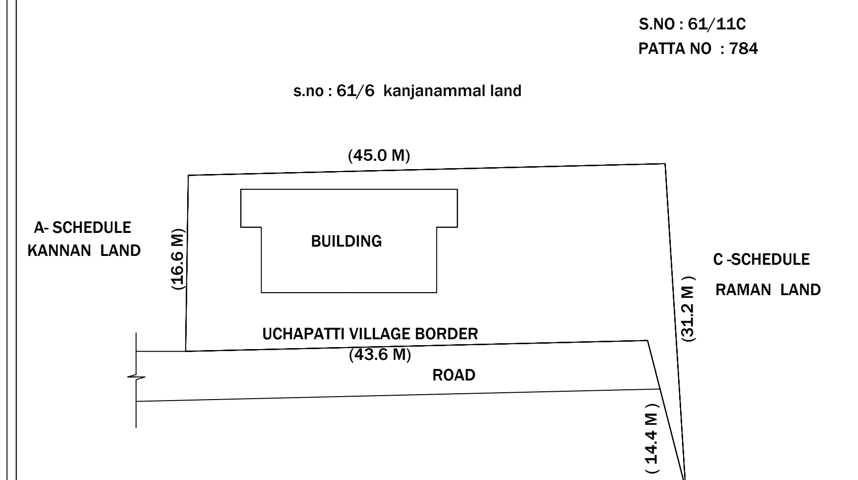
SITE PLAN
