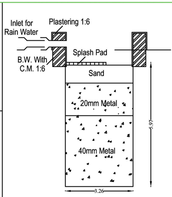
RAIN WATER PERCOLATION PIT
