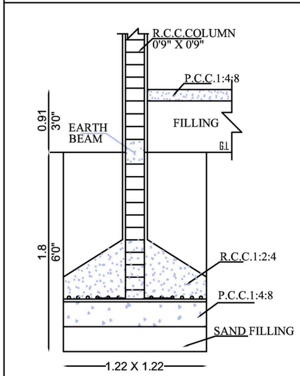
FOUNDATION DETAILS
