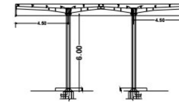
CANOPY DETAIL
