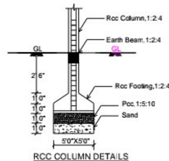
RCC COLUMN DETAILS
