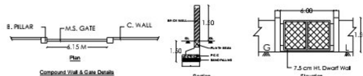
Compound Wall & Gate Details
