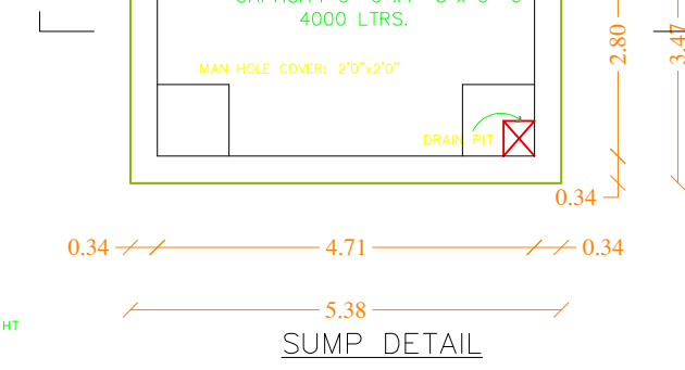
U.G. SUMP CAPACITY 6'-6"x4'-0"x 6'-0" 4000 LTRS.
