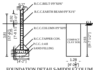
FOUNDATION DETAILS-MIDDLE COLUMN
