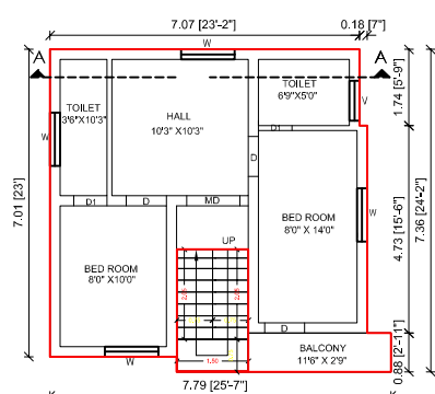
EXG.FIRST FLOOR PLAN
