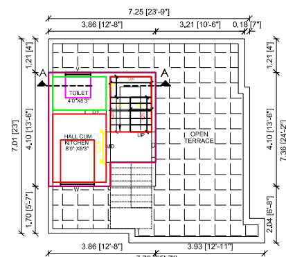
PRO.SECOND FLOOR PLAN
