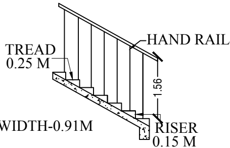
STAIRCASE DETAILS
