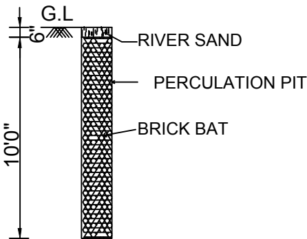
PERCULATION PIT
