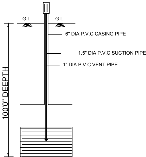
BORE WELL
