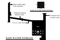
RAIN WATER STORAGE
