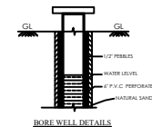
BORE WELL DETAILS
