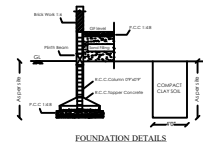
FOUNDATION DETAILS
