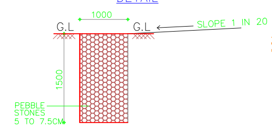
SECTION OF PEBBLE TRENCH
