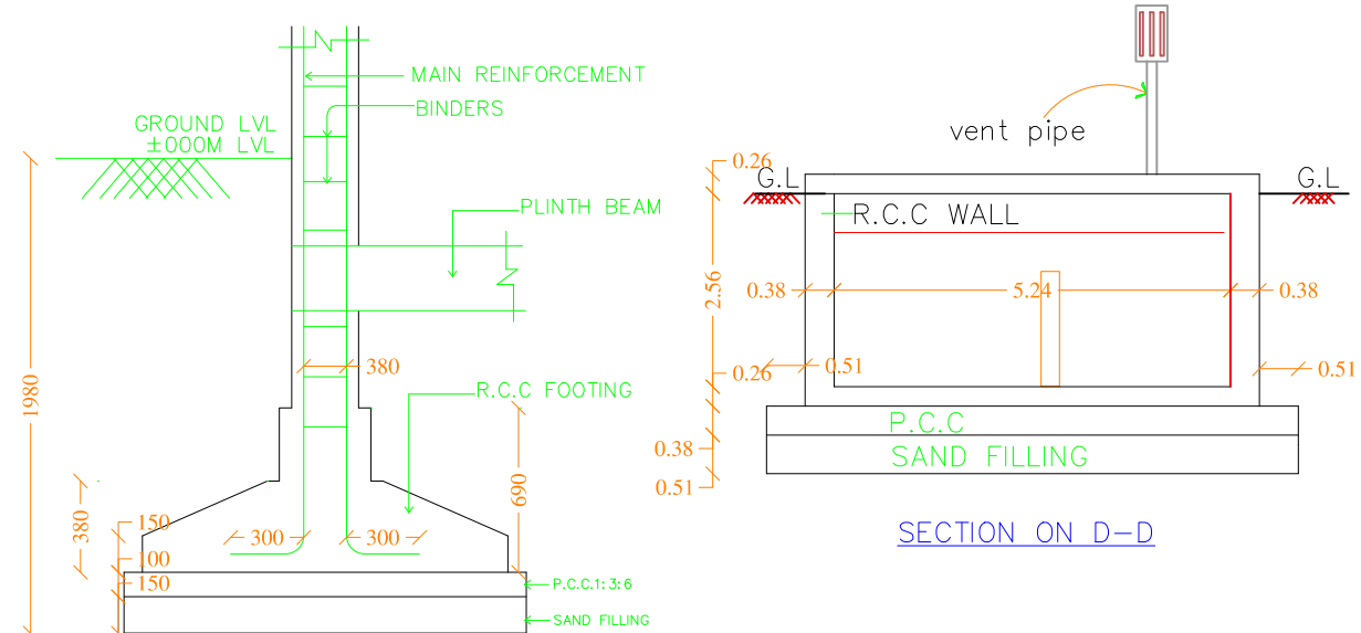
TYPICAL SECTION OF R.C.C. COLUMN FOUNDATION
