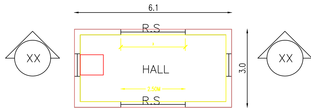
PROPOSED GROUND FLOOR
