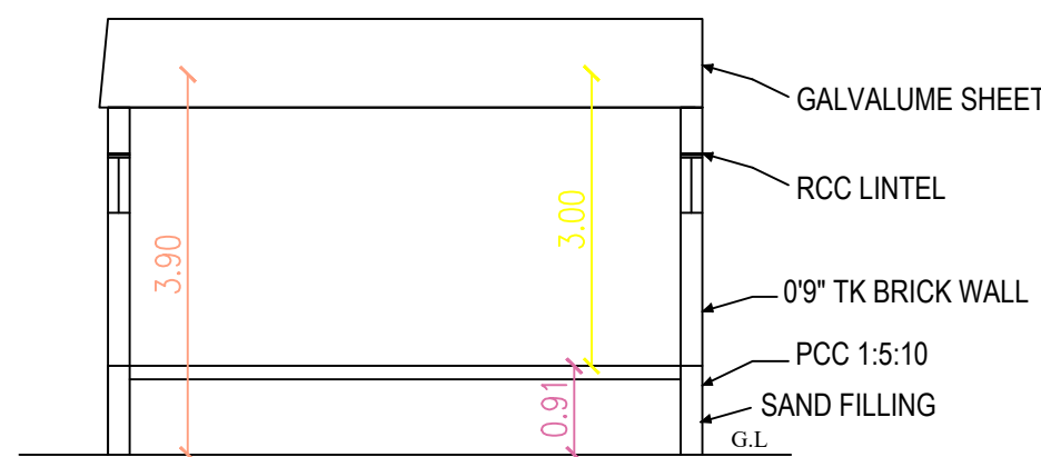
SECTION CUTTING XX
