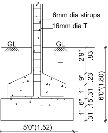
COLUMN FOUNDATION DETAIL
