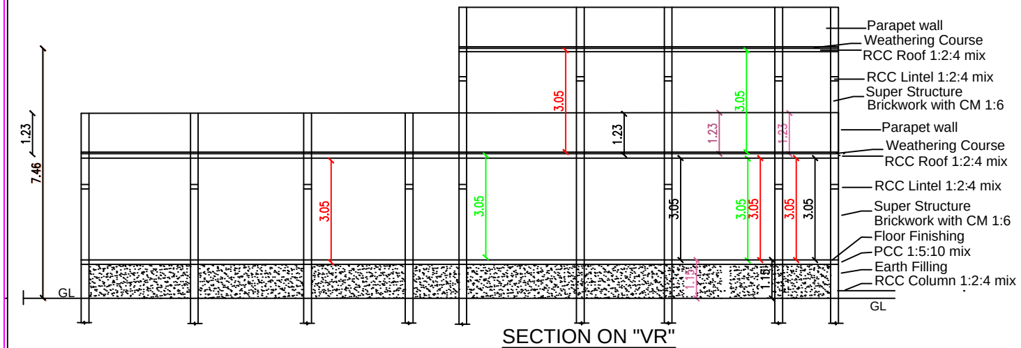
SECTION ON "VR"
