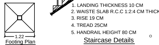
Staircase Details
