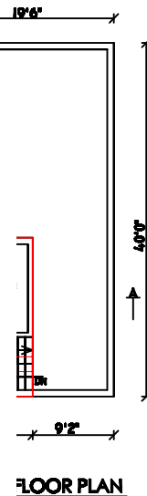
FLOOR PLAN
