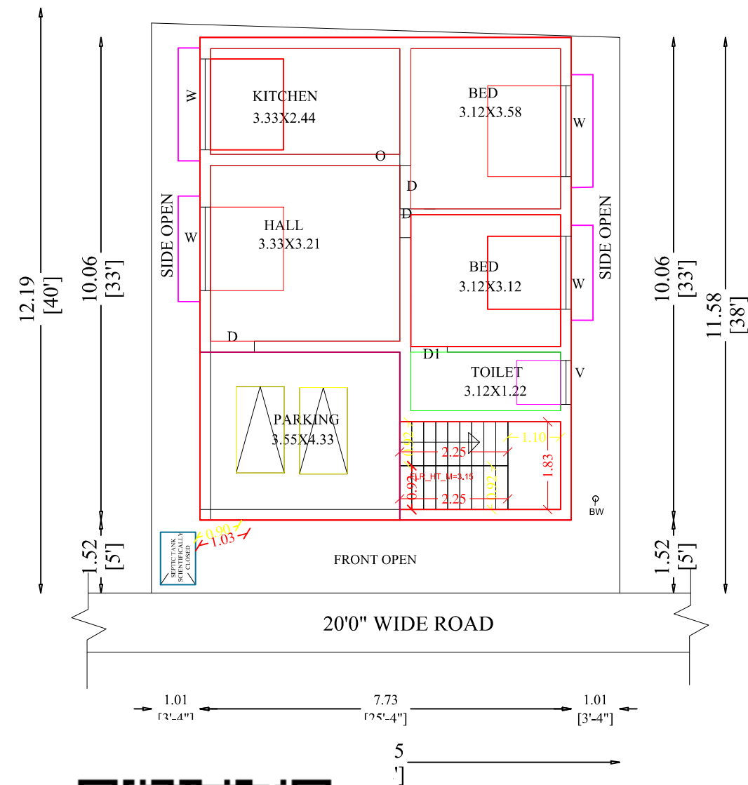
FLOOR PLAN
