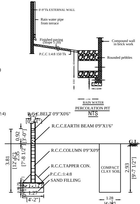
FOUNDATION DETAILS-MIDDLE COLUMN
