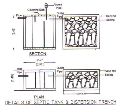
DETAILS OF SEPTIC TANK & DISPERSION TRENCH
