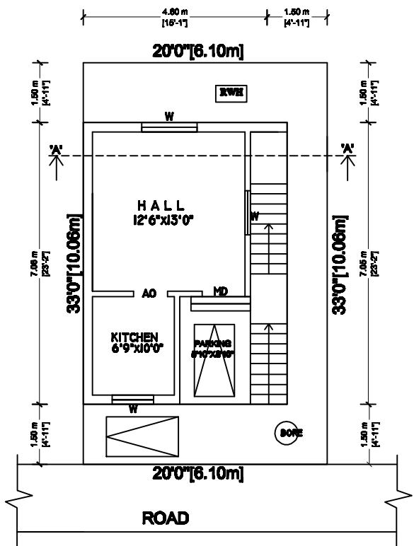
JND FLOOR PLAN
