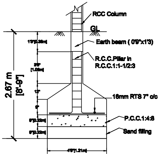
FOUNDATION DETAILS
