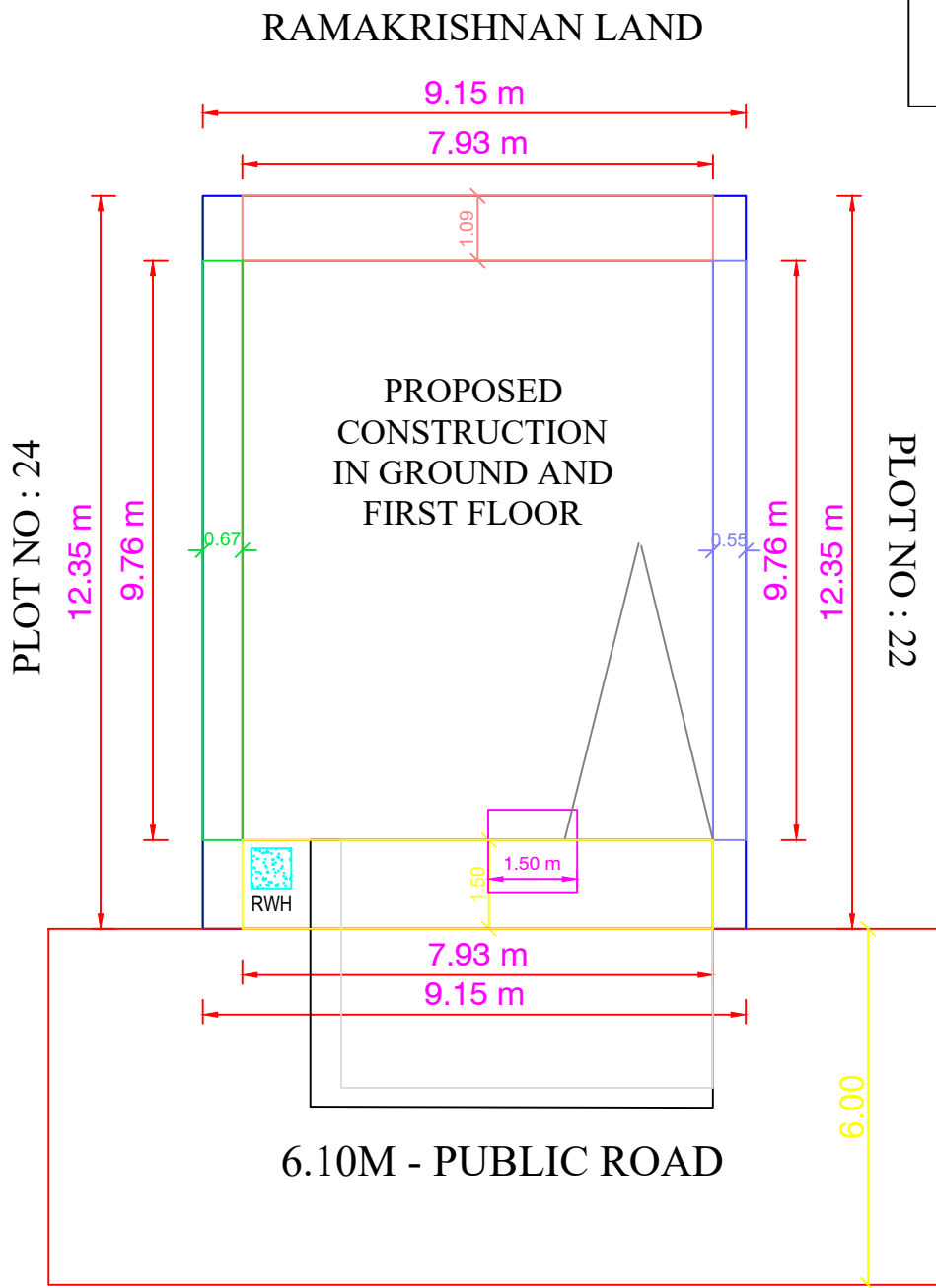
SITE PLAN
