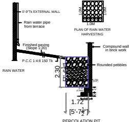
PERCOLATION PIT
