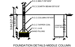
FOUNDATION DETAILS-MIDDLE COLUMN
