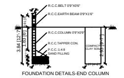
FOUNDATION DETAILS-END COLUMN
