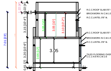
SECTION ON B-B
