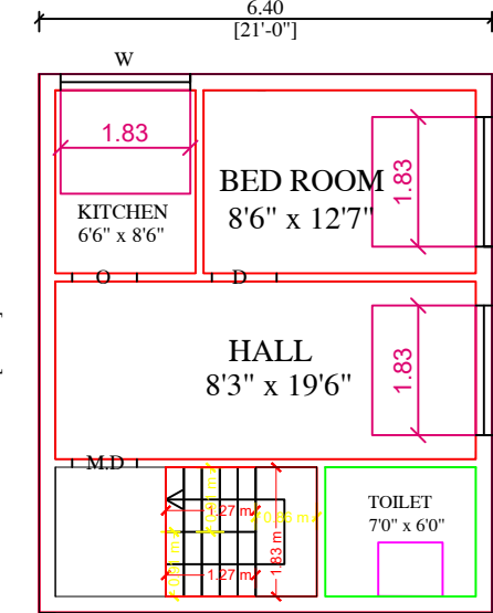
PRO. SECOND FLOOR PLAN
