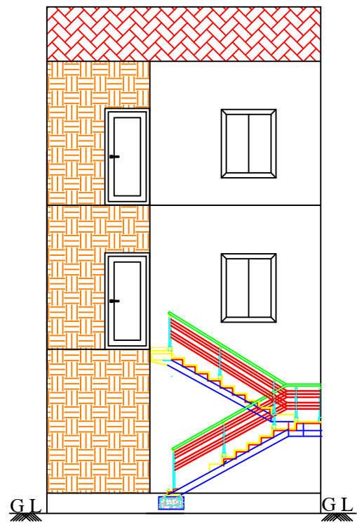
FRONT ELEVATION
