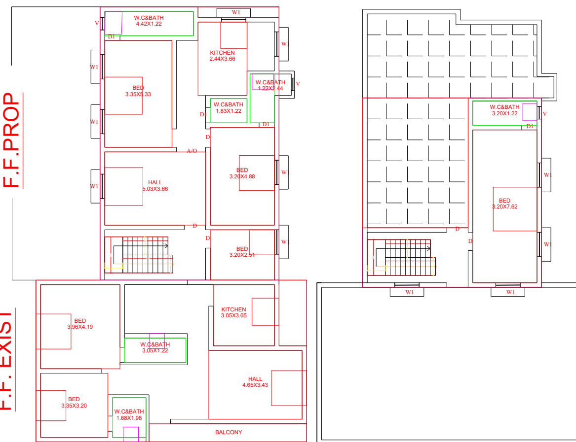
FIRST FLOOR EXISTING & FIRST FLOOR ADDITIONAL
