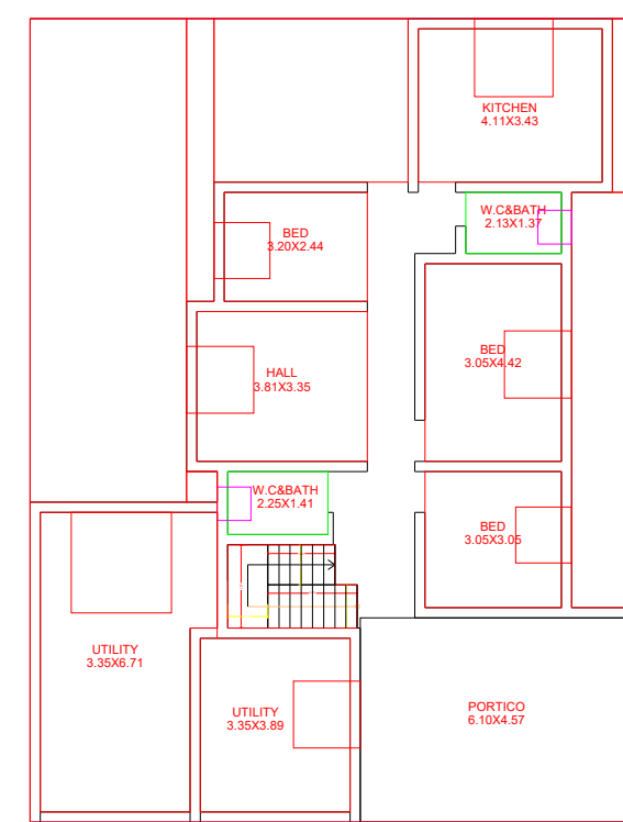
GROUND FLOOR EXISTING
