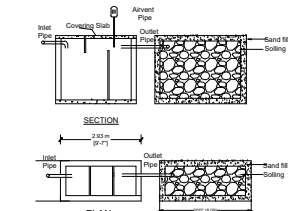
DETAILS OF SEPTIC TANK & DISPERSION TRENCH
