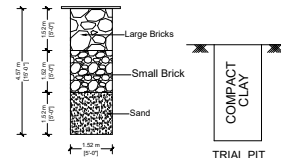
SECTION OF RAIN WATER COLLECTION PITS (NTS)
