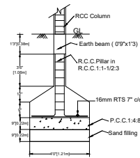
FOUNDATION DETAILS
