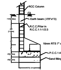
FOUNDATION DETAILS
