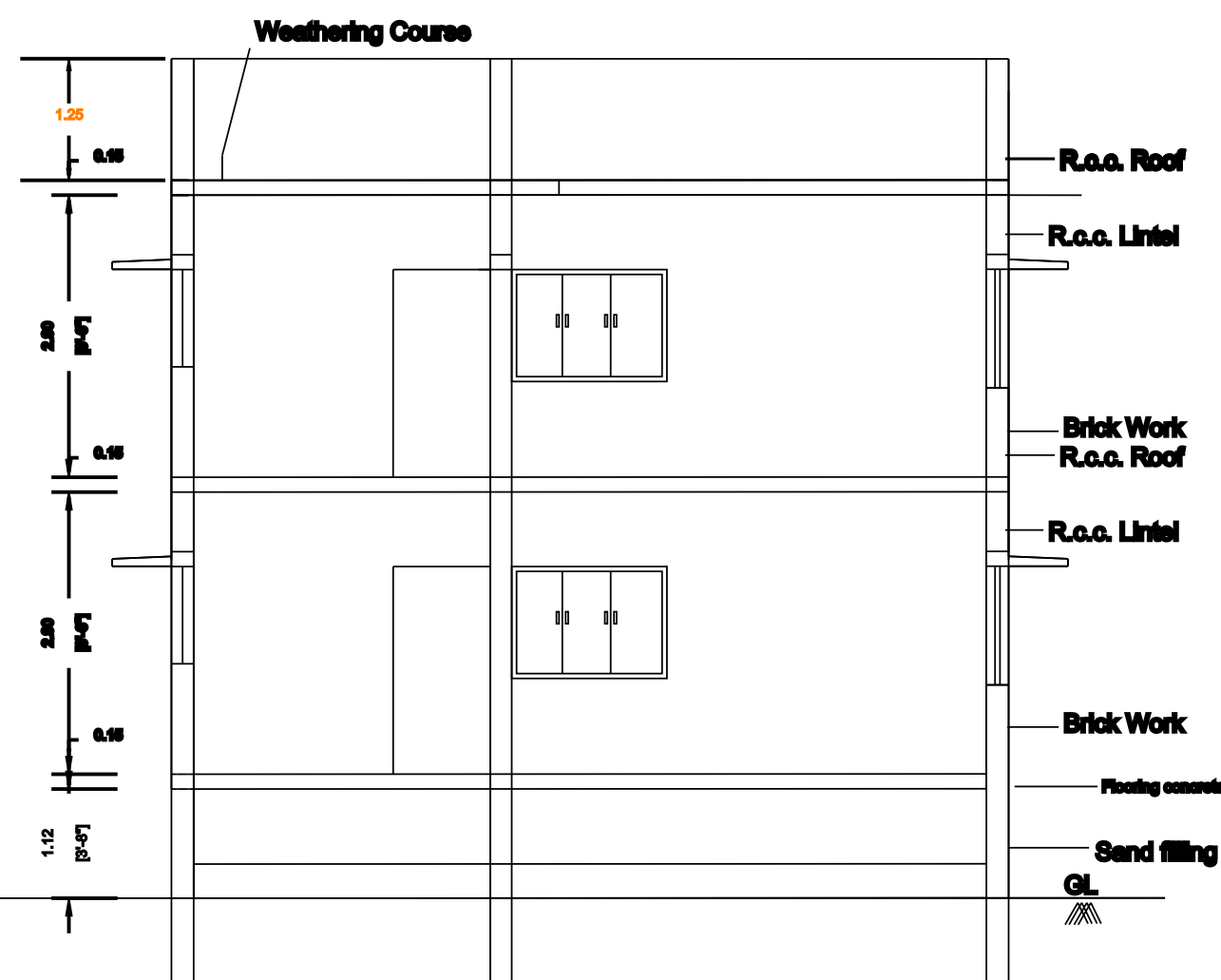
SECTION- BB
