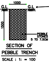
SECTION OF PEBBLE TRENCH
