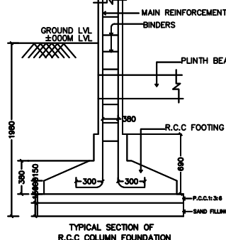
TYPICAL SECTION OF R.C.C COLUMN FOUNDATION
