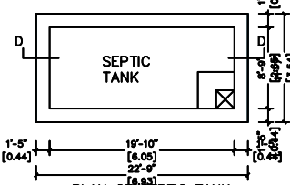
PLAN OF SEPTIC TANK
