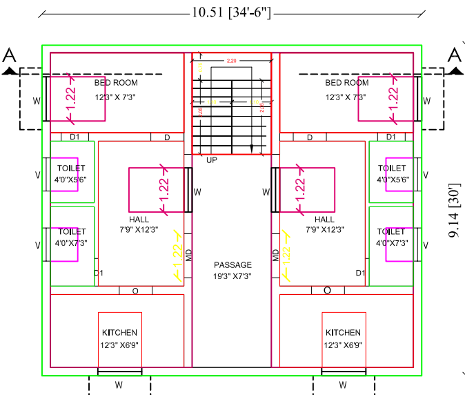
TYPICAL FLOOR PLAN ( FIRST, SECOND,THIRD)
