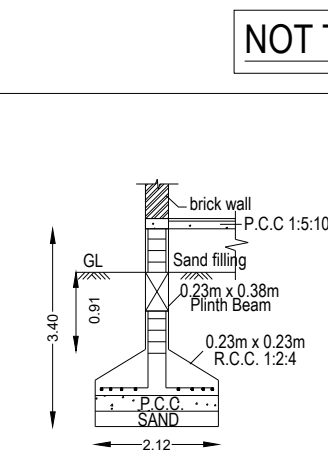
FOUNDATION DETAILS
