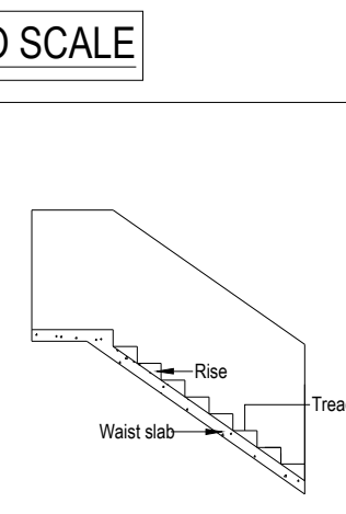
DETAILS OF STAIR CASE
