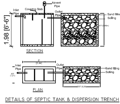
DETAILS OF SEPTIC TANK & DISPERSION TRENCH
