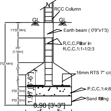
FOUNDATION DETAILS
