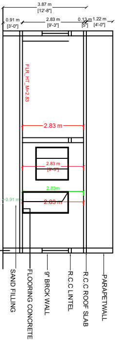
SECTION ON 'A-A'
