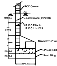
FOUNDATION DETAILS
