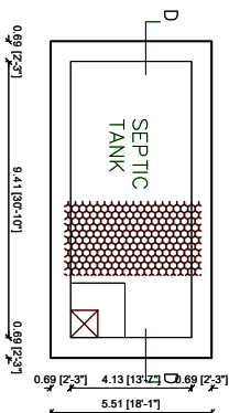
PLAN OF SEPTIC TANK SCALE 1"=2'0"
