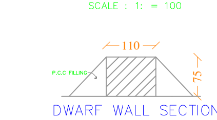
SECTION OF PEBBLE TRENCH
