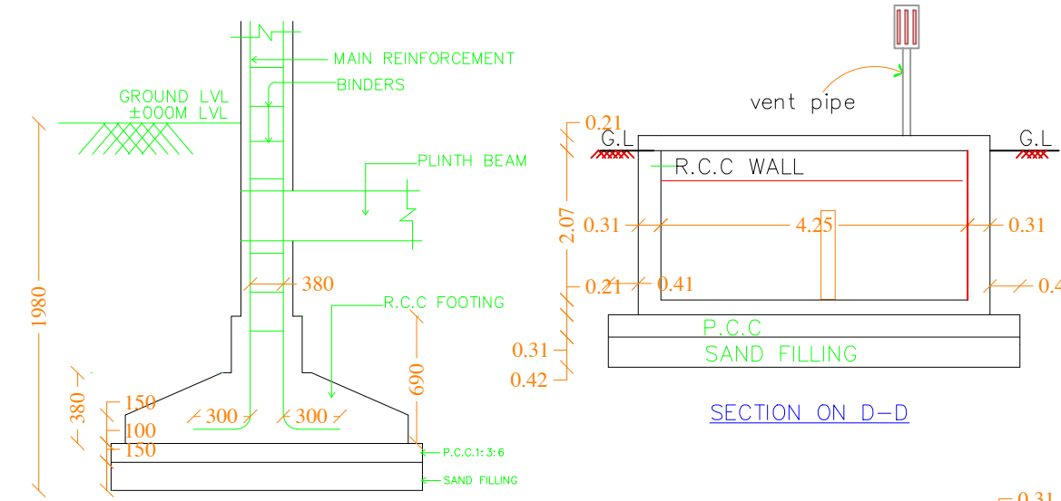
SECTION ON D-D
