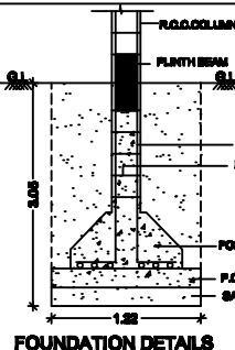
FOUNDATION DETAILS
