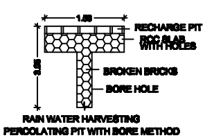
RAIN WATER HARVESTING PERCOLATING PIT WITH BORE METHOD
