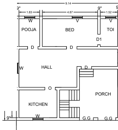
PROPOSED F.F PLAN
