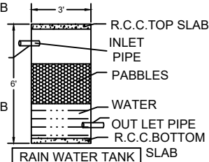
RAIN WATER TANK
